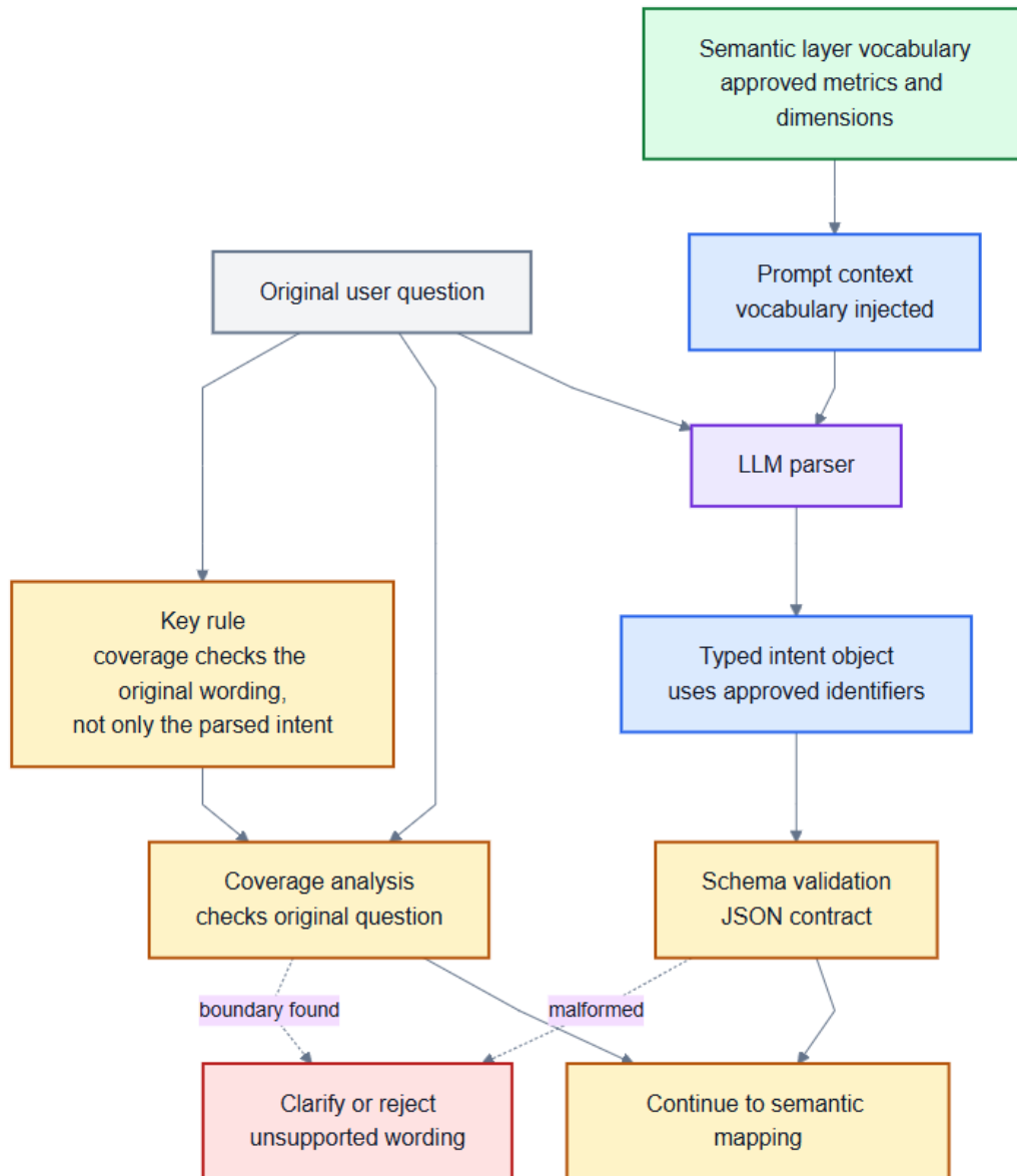
Figure 4: Vocabulary injection and original-question coverage workflow
